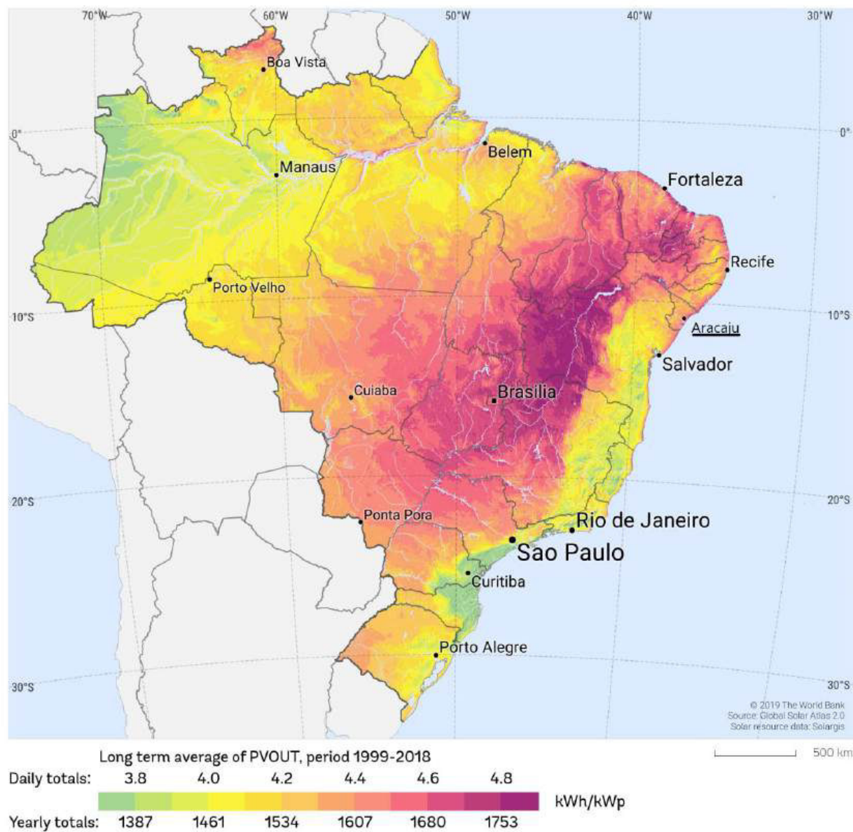
Figure A8.2 Photovoltaic Power Potential in Brazil, annual average.
